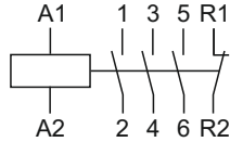
ST25-31/24, ST25-31, ST40-31, ST63-31
