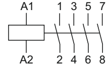
ST25-04, ST25-40/24, ST40-40/24, ST40-40, ST63-40, ST63-40/24, ST100-40, ST25-40-24AC/DC, ST63-40-24AC/DC
